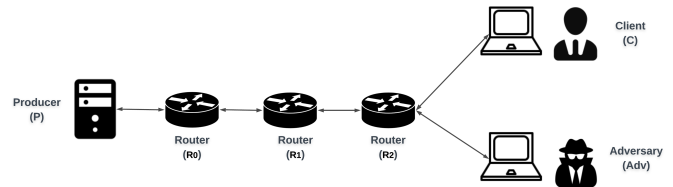
Fig. 1. Topology
