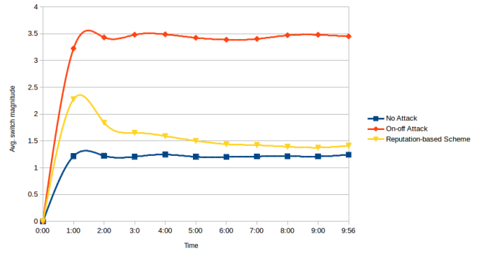
Fig. 3. Reputation-based countermeasure efficiency: Avg. magnitude
